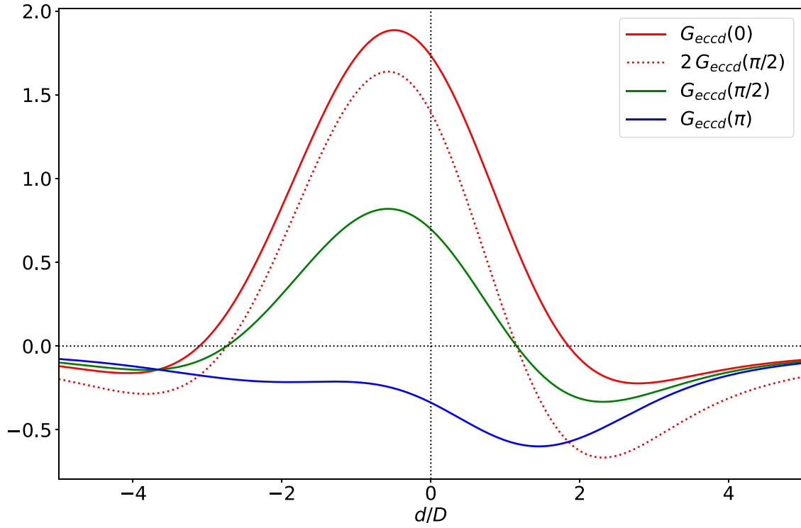
Figure 19. The integral G_{\text{eccd}}(\Delta\zeta) evaluated as a function of d/D at \Delta\zeta = 0, \pi/2 , and \pi for an island of full width W = 4.0D and asymmetry parameter \delta = 0.5 . The dotted curve shows the integral when the driven current profile is independent of \zeta .
