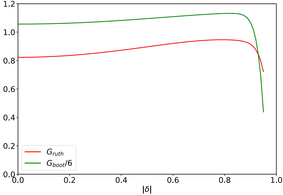
Figure 16. The integrals G_{\text{ruth}} and G_{\text{boot}}/6 evaluated as functions of the modulus of the island asymmetry parameter, |\delta| .
