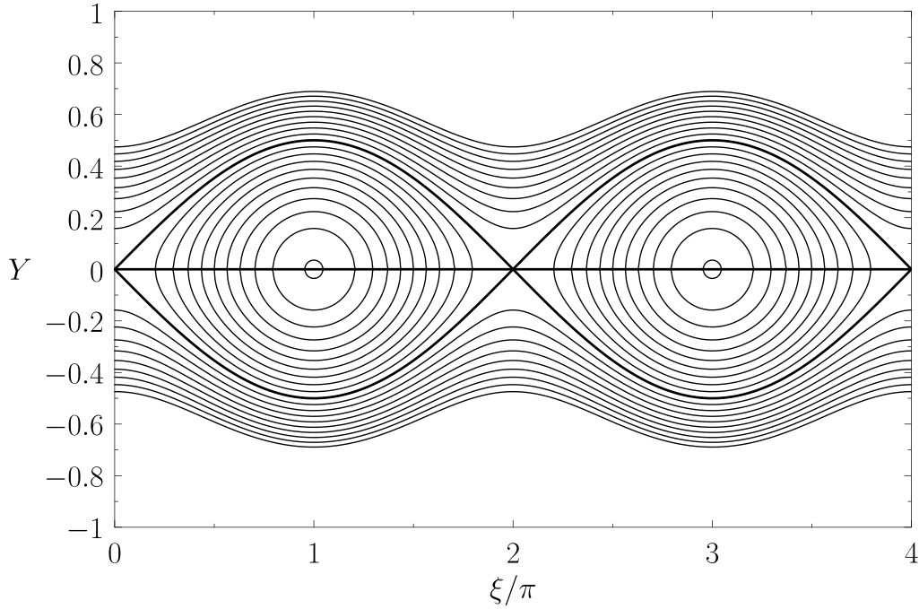
Figure 12. The thin solid curves show the contours of \Omega(Y, \xi) evaluated for \delta = 0.5 . The thick solid lines show the magnetic separatrix (upper and lower curves) and the contour Y = 0 (middle curve). Reprinted from [46], with the permission of AIP Publishing.
