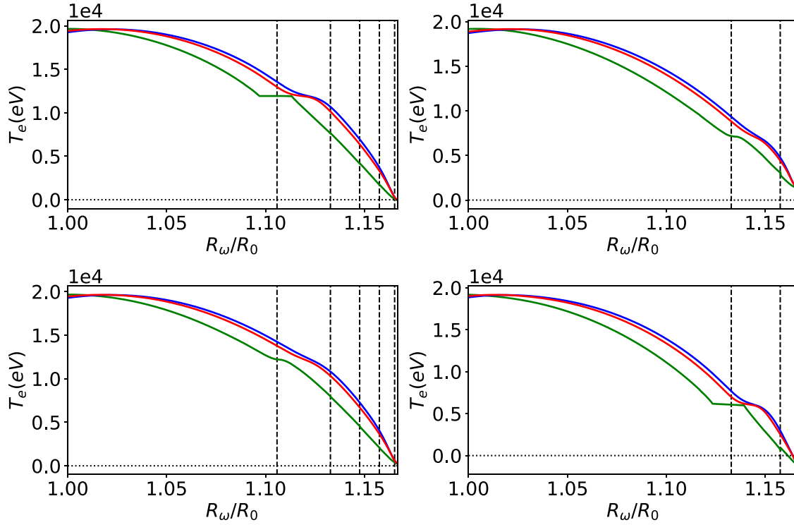
Figure 8. Total electron temperature along the ECE chord (green curves) and the perturbed temperature inferred by the relativistically downshifted and broadened 1st harmonic O-mode (blue curves) and 2nd harmonic X-mode (red curves) ECE diagnostic for a 3, 2 NTM (left panels) and a 2, 1 NTM (right panels) of island width W = 0.1 a in the model plasma equilibrium pictured in figures 1 and 2. The total temperatures are calculated at two different toroidal angles (top and bottom panels). The vertical dashed lines show the locations of the rational surfaces.
