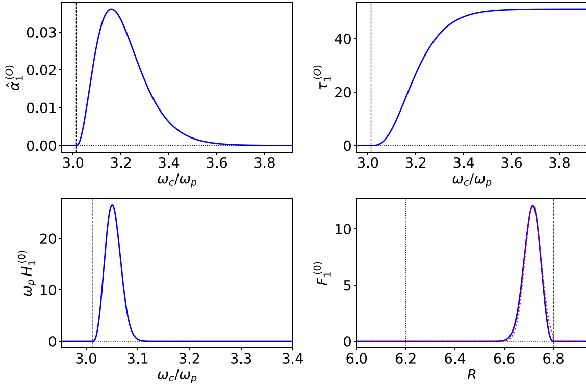
Figure 21. The normalized absorption coefficient (top left), optical depth (top right), normalized spectral convolution function (bottom left), and spatial convolution function (bottom right), for 1st harmonic O-mode ECE from an ITER-like plasma characterized by T_e = 10\text{keV} , n_e = 2.5 \times 10^{19}\text{m}^{-3} (at the 1st harmonic cyclotron resonance), B_0 = 5.3\text{T} , R_0 = 6.2\text{m} , and R_\omega = 6.8\text{m} . The vertical dashed lines show the location of the 1st harmonic cyclotron resonance. The vertical dotted line (in the bottom right panel) shows the location of the magnetic axis. The dotted red curve in the bottom right panel is a fit to the true spatial convolution function (shown in blue).
