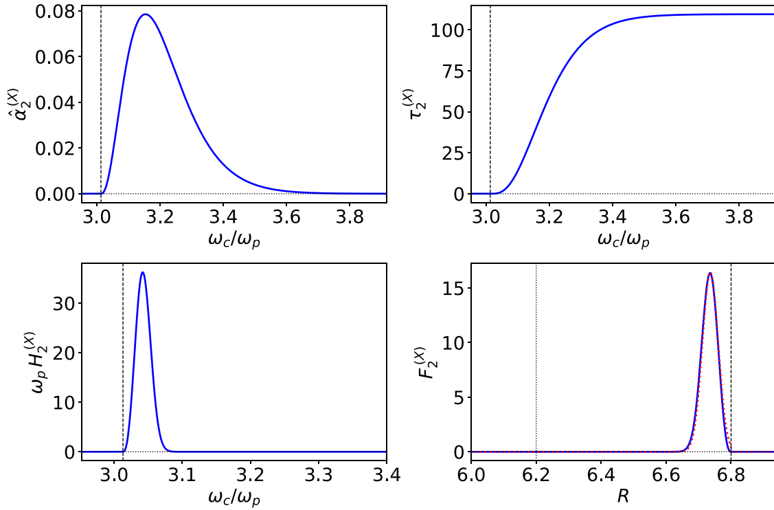
Figure 22. The normalized absorption coefficient (top left), optical depth (top right), normalized spectral convolution function (bottom left), and spatial convolution function (bottom right), for 2nd harmonic X-mode ECE from an ITER-like plasma characterized by T_e = 10\text{ keV} , n_e = 2.5 \times 10^{19}\text{ m}^{-3} (at the 2nd harmonic cyclotron resonance), B_0 = 5.3\text{ T} , R_0 = 6.2\text{ m} , and R_\omega = 6.8\text{ m} . The vertical dashed lines show the location of the 2nd harmonic cyclotron resonance. The vertical dotted line (in the bottom right panel) shows the location of the magnetic axis. The dotted red curve in the bottom right panel is a fit to the true spatial convolution function (shown in blue).
