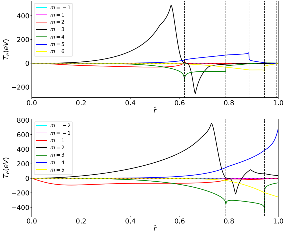
Figure 3. Harmonics of the perturbed electron temperature associated with a 3, 2 (top panel) and a 2, 1 (bottom panel) NTM of island width W = 0.1a in the example plasma equilibrium pictured in figures 1 and 2. The harmonics all have the same toroidal mode number as the NTM. The vertical dashed lines show the positions of the rational surfaces.
