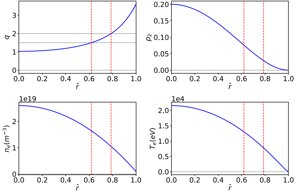
Figure 2. The safety-factor, normalized pressure, electron number density, and electron temperature profiles for the example equilibrium pictured in figure 1. The vertical red lines show the locations of the q = 3/2 and q = 2 surfaces.
