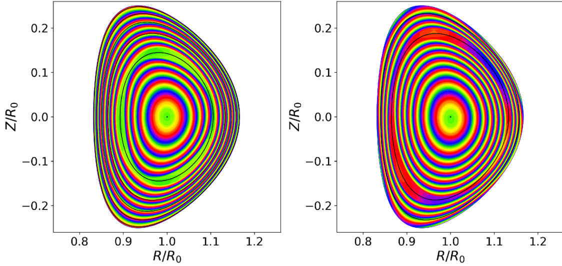
Figure 5. Total electron temperature at a particular toroidal angle (which is the same as that in figure 4) associated with a 3, 2 (left panel) and a 2, 1 (right panel) NTM of island width W = 0.1a in the example plasma equilibrium pictured in figures 1 and 2. The black curves show the locations of the rational surfaces. The black dot shows the location of the magnetic axis.
