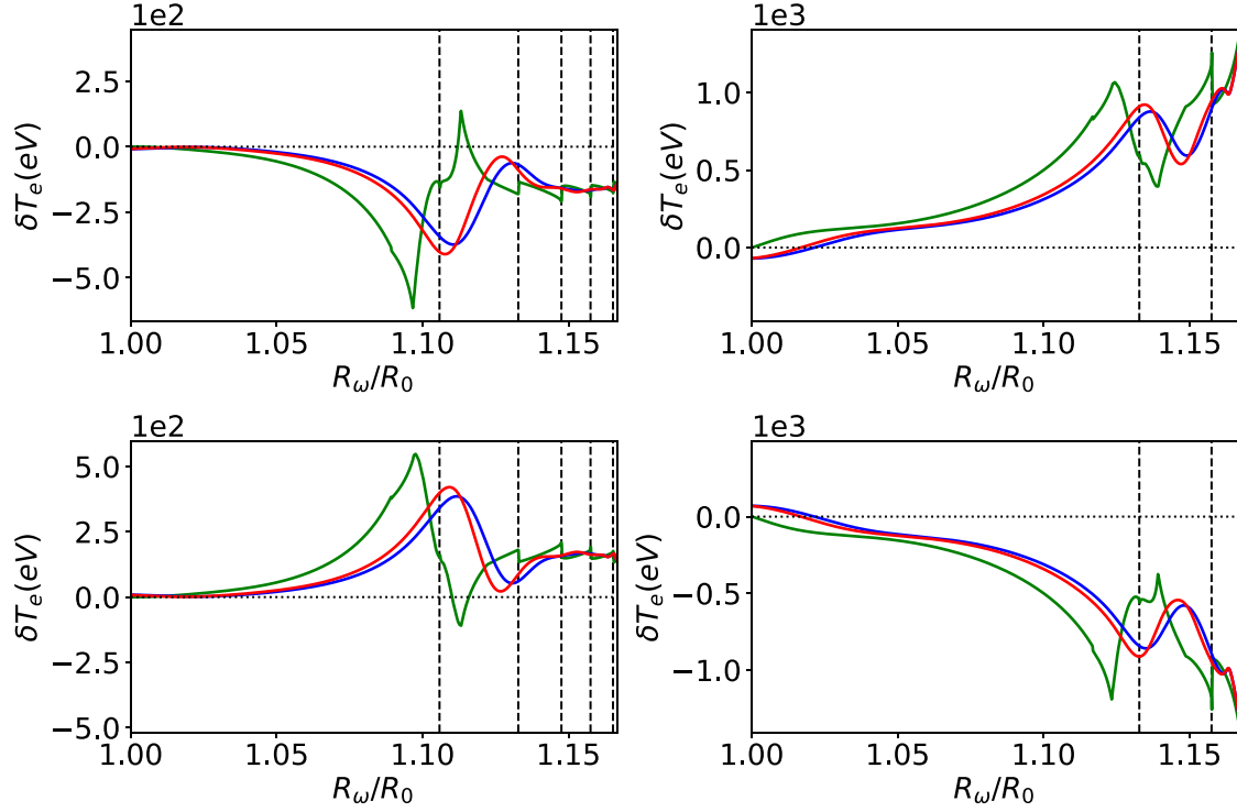
Figure 7. Perturbed electron temperature along the ECE measurement chord (green curves) and the perturbed temperature inferred by the relativistically downshifted and broadened 1st harmonic O-mode (blue curves) and 2nd harmonic X-mode (red curves) ECE diagnostic for a 3, 2 NTM (left panels) and a 2, 1 NTM (right panels) of island width W = 0.1a in the model plasma equilibrium pictured in figures 1 and 2. The perturbed temperatures are calculated at two different toroidal angles (top and bottom panels). The vertical dashed lines show the locations of the rational surfaces.
