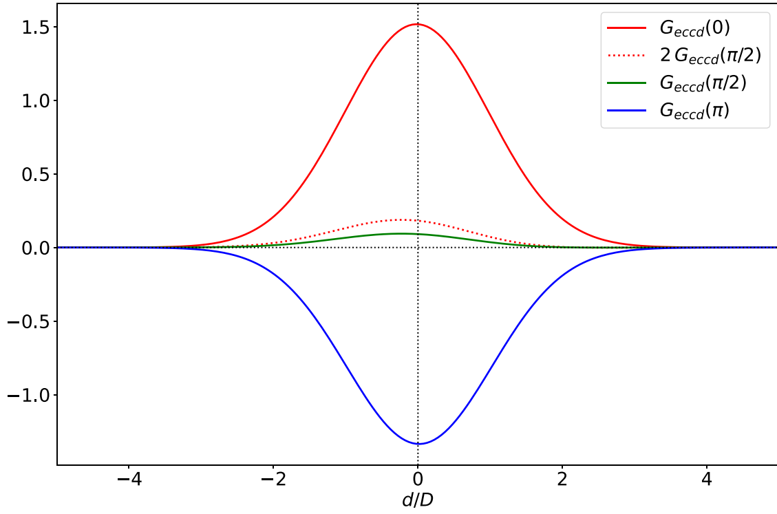
Figure 17. The integral G_{\text{eccd}}(\Delta\zeta) evaluated as a function of d/D at \Delta\zeta = 0, \pi/2 , and \pi for an island of full width W = 0.1D and asymmetry parameter \delta = 0.5 . The dotted curve shows the integral when the driven current profile is independent of \zeta .
