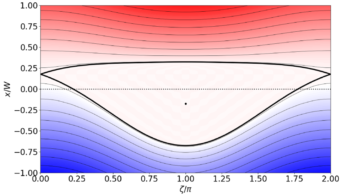
Figure 15. Contours of the normalized electron temperature profile, \tilde{T}(x/W, \zeta) , in the vicinity of an asymmetric magnetic island characterized by \delta = 0.5 . The thick solid line shows the magnetic separatrix, the dotted line shows the rational surface, and the black dot shows the island O-point.
