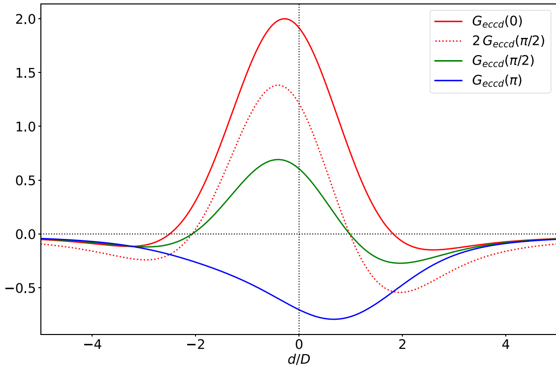
Figure 18. The integral G_{\text{eccd}}(\Delta\zeta) evaluated as a function of d/D at \Delta\zeta = 0, \pi/2 , and \pi for an island of full width W = 2.0D and asymmetry parameter \delta = 0.5 . The dotted curve shows the integral when the driven current profile is independent of \zeta .
