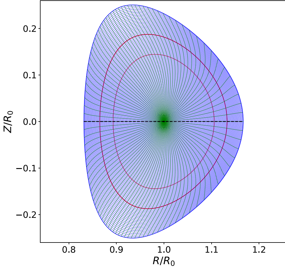
Figure 1. The blue and green curves show surfaces of constant r and \theta , respectively, for an ITER-like example plasma equilibrium characterized by B_0 = 5.3 T, R_0 = 6.2 m, a = 0.2 , H_2(1) = 1.0 , and H_3(1) = 0.5 . The red curves show the locations of the q = 3/2 and q = 2 surfaces. The dashed black line shows the location of the ECE measurement chord.
