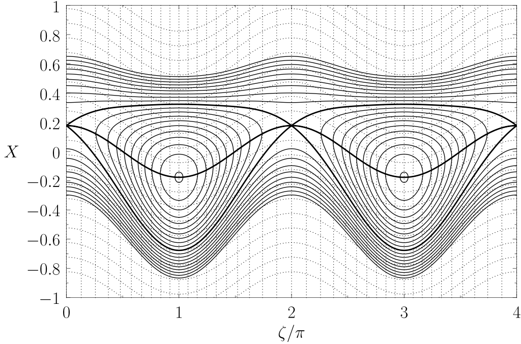
Figure 11. The thin solid curves show the contours of \Omega(X, \zeta) evaluated for \delta = 0.5 . The thick solid lines show the magnetic separatrix (upper and lower curves) and the contour Y = 0 (middle curve). The curved dotted lines show equally-spaced contours of Y , whereas the vertical dotted lines show equally-spaced contours of \xi . Reprinted from [46], with the permission of AIP Publishing.
