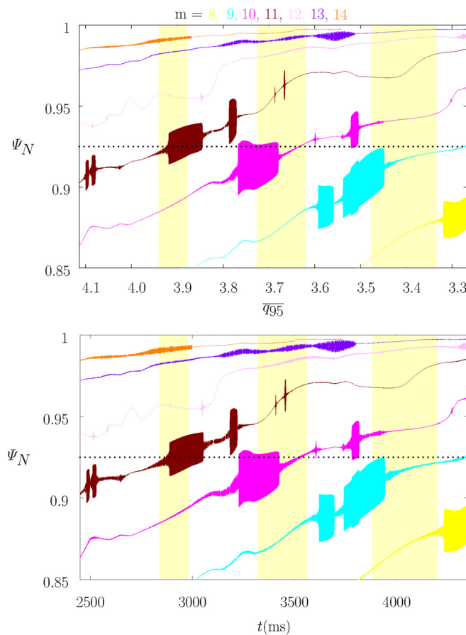
FIG. 7. Top panel: Density flattening widths associated with induced n=3 magnetic island chains as functions of the least squares linear fit to q_{95} vs time in DIII-D discharge #145380, assuming that the natural frequency is determined by nonlinear island physics. Bottom panel: Electron temperature flattening widths associated with induced n=3 magnetic island chains as functions of time in DIII-D discharge #145380, assuming that the natural frequency is determined by nonlinear island physics. The yellow, cyan, magenta, brown, pink, purple, and orange areas correspond to m=8, 9, 10, 11, 12, 13 , and 14 , respectively. The yellow vertical bands indicate the ELM-suppression/mitigation windows. The horizontal dotted lines indicate the top of the pedestal, \Psi_N = 0.925 .
