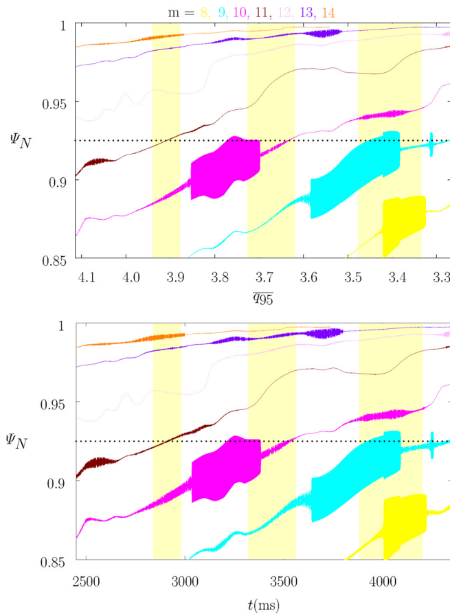
FIG. 13. Top panel: Density flattening widths associated with induced n=3 magnetic island chains as functions of the least squares linear fit to q_{95} vs time in DIII-D discharge #145380, assuming that the natural frequency is determined by linear layer physics. Bottom panel: Electron temperature flattening widths associated with induced n=3 magnetic island chains as functions of time in DIII-D discharge #145380, assuming that the natural frequency is determined by linear layer physics. The yellow, cyan, magenta, brown, pink, purple, and orange areas correspond to m=8, 9, 10, 11, 12, 13 , and 14 , respectively. The yellow vertical bands indicate the ELM-suppression/mitigation windows. The horizontal dotted lines indicate the top of the pedestal, \Psi_N = 0.925 .
