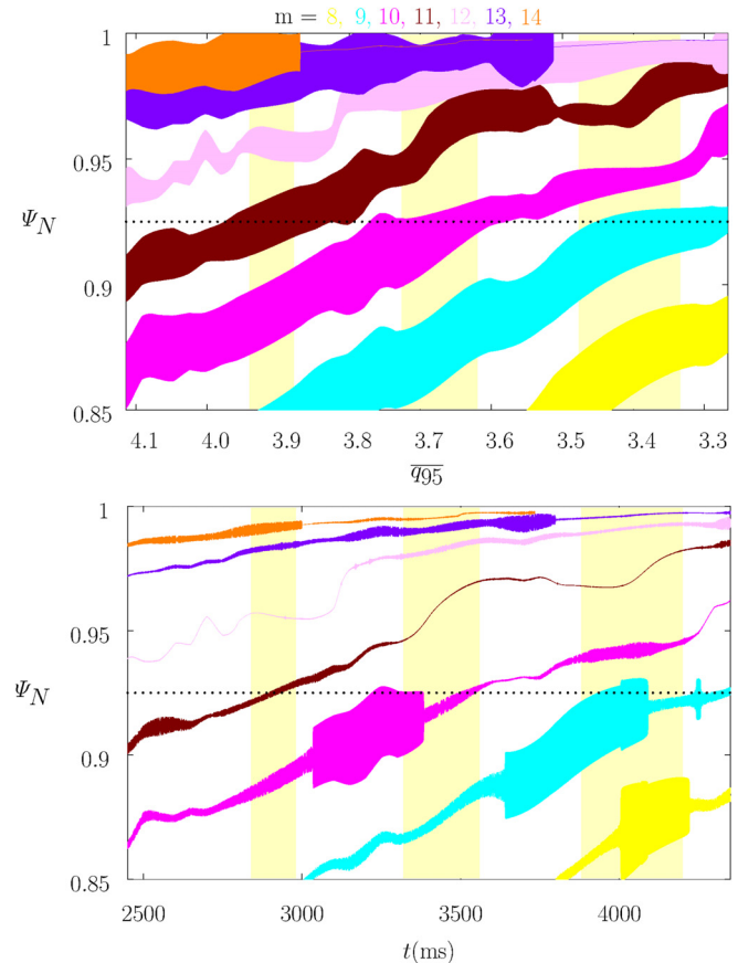
FIG. 12. Top panel: n = 3 vacuum island widths as functions of the least squares linear fit to q_{95} vs time in DIII-D discharge #145380, assuming that the natural frequency is determined by linear layer physics. Bottom panel: n = 3 island widths as functions of time in DIII-D discharge #145380, assuming that the natural frequency is determined by linear layer physics. The yellow, cyan, magenta, brown, pink, purple, and orange areas correspond to m = 8, 9, 10, 11, 12, 13 , and 14 , respectively. The yellow vertical bands indicate the ELM-suppression/mitigation windows. The horizontal dotted lines indicate the top of the pedestal, \Psi_N = 0.925 .
