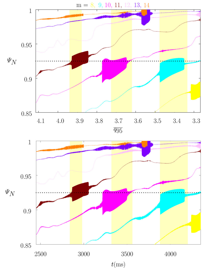
FIG. 10. Top panel: Density flattening widths associated with induced n = 3 magnetic island chains as functions of the least squares linear fit to q_{95} vs time in DIII-D discharge #145380, assuming that the natural frequency is determined by the local \mathbf{E} \times \mathbf{B} velocity. Bottom panel: Electron temperature flattening widths associated with induced n = 3 magnetic island chains as functions of time in DIII-D discharge #145380, assuming that the natural frequency is determined by the local \mathbf{E} \times \mathbf{B} velocity. The yellow, cyan, magenta, brown, pink, purple, and orange areas correspond to m = 8, 9, 10, 11, 12, 13 , and 14, respectively. The yellow vertical bands indicate the ELM-suppression/mitigation windows. The horizontal dotted lines indicate the top of the pedestal, \Psi_N = 0.925 .
