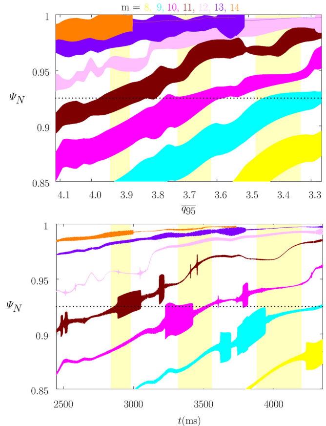
FIG. 6. Top panel: Full n = 3 vacuum island widths as functions of the least squares linear fit to q_{95} vs time in DIII-D discharge #145380. Bottom panel: Full n = 3 island widths as functions of time in DIII-D discharge #145380, assuming that the natural frequency is determined by nonlinear island physics. The yellow, cyan, magenta, brown, pink, purple, and orange areas correspond to m = 8, 9, 10, 11, 12, 13 , and 14 , respectively. The yellow vertical bands indicate the ELM-suppression/mitigation windows. The horizontal dotted lines indicate the top of the pedestal, \Psi_N = 0.925 .
