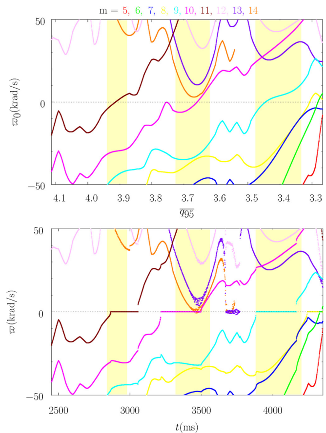
FIG. 8. Top panel: n=3 natural frequencies, in the absence of RMP, as functions of the least squares linear fit to q_{95} vs time in DIII-D discharge #145380, assuming that the natural frequency is determined by the local \mathbf{E} \times \mathbf{B} velocity. Bottom panel: n=3 natural frequencies, in the presence of RMP, as functions of time in DIII-D discharge #145380, assuming that the natural frequency is determined by the local \mathbf{E} \times \mathbf{B} velocity. The red, green, blue, yellow, cyan, magenta, brown, pink, purple, and orange curves correspond to m=5, 6, 7, 8, 9, 10, 11, 12, 13 , and 14 , respectively. The yellow vertical bands indicate the ELM-suppression/mitigation windows.
