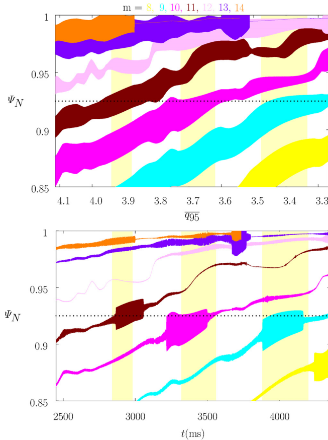
FIG. 9. Top panel: n = 3 vacuum island widths as functions of the least squares linear fit to q_{95} vs time in DIII-D discharge #145380, assuming that the natural frequency is determined by the local \mathbf{E} \times \mathbf{B} velocity. The yellow, cyan, magenta, brown, pink, purple, and orange areas correspond to m = 8, 9, 10, 11, 12, 13 , and 14, respectively. The yellow vertical bands indicate the ELM-suppression/mitigation windows. The horizontal dotted lines indicate the top of the pedestal, \Psi_N = 0.925 .
