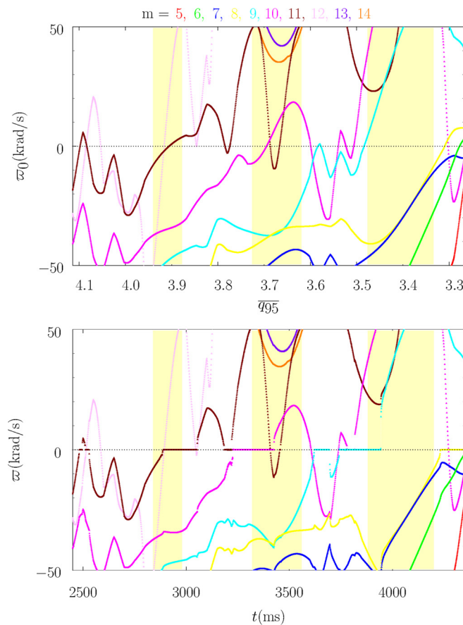
FIG. 5. Top panel: n = 3 natural frequencies, in the absence of RMP, as functions of the least squares linear fit to q_{95} vs time in DIII-D discharge #145380, assuming that the natural frequency is determined by nonlinear island physics. Bottom panel: n = 3 natural frequencies, in the presence of RMP, as functions of time in DIII-D discharge #145380, assuming that the natural frequency is determined by nonlinear island physics. The red, green, blue, yellow, cyan, magenta, brown, pink, purple, and orange curves correspond to m = 5, 6, 7, 8, 9, 10, 11, 12, 13 , and 14 , respectively. The yellow vertical bands indicate the ELM-suppression windows.
