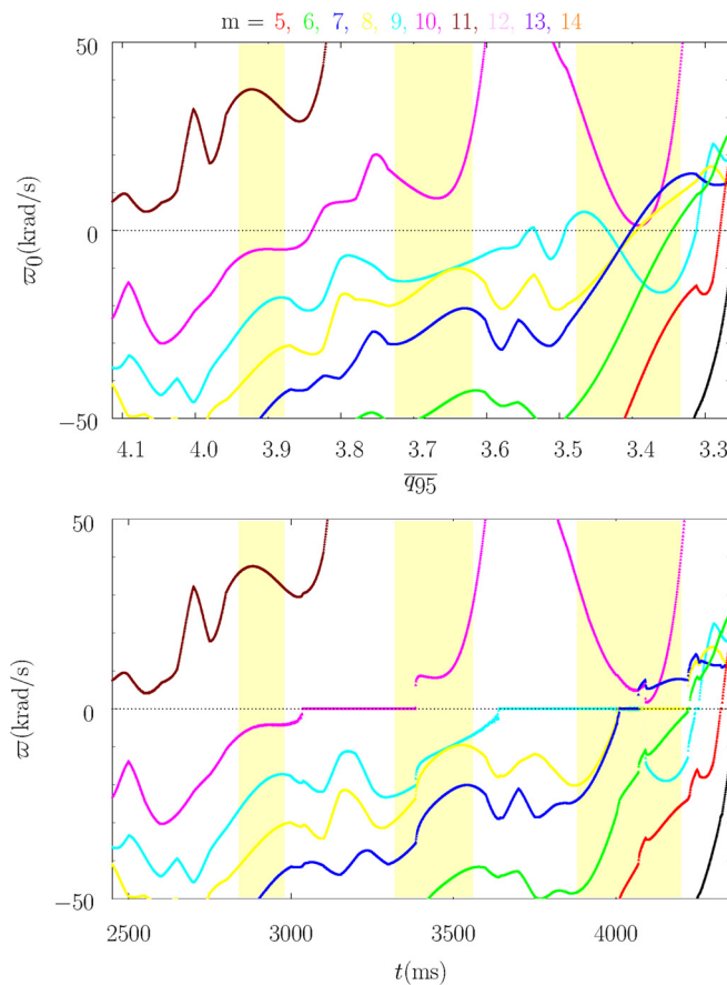
FIG. 11. Top panel: n = 3 natural frequencies, in the absence of RMP, as functions of the least squares linear fit to q_{95} vs time in DIII-D discharge #145380, assuming that the natural frequency is determined by linear layer physics. Bottom panel: n = 3 natural frequencies, in the presence of RMP, as functions of time in DIII-D discharge #145380, assuming that the natural frequency is determined by linear layer physics. The black, red, green, blue, yellow, cyan, magenta, brown, purple, and orange curves correspond to m = 4, 5, 6, 7, 8, 9, 10, 11, 13 , and 14 , respectively. The yellow vertical bands indicate the ELM-suppression/mitigation windows.
