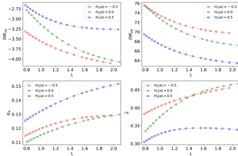
FIG. 7. The no-wall perturbed potential energy, \delta W_{nw} , the perfect-wall perturbed potential energy, \delta W_{pw} , the wall parameter, \alpha_w , and the normalized thin-wall growth-rate, \hat{\gamma} , of the vertical mode, plotted as functions of the plasma self-inductance, l_i , for plasma equilibria characterized by \epsilon = 0.1 , H_2(a) = 1 , q(a) = 3.6 , p_2 = 0.05 , \nu_p = 2.5 , b_w = 1.1 , and various different values of H_3(a) .
