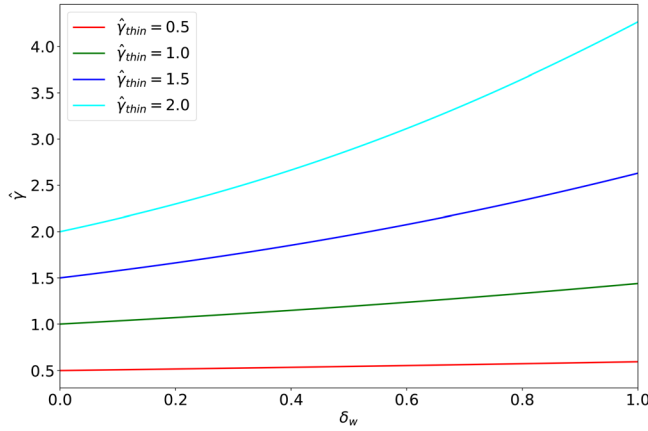
FIG. 8. Variation of the true normalized resistive wall mode growth-rate, \hat{\gamma} , with the wall thickness parameter, \delta_w , for various values of the thin-wall normalized growth-rate, \hat{\gamma}_{thin} .
