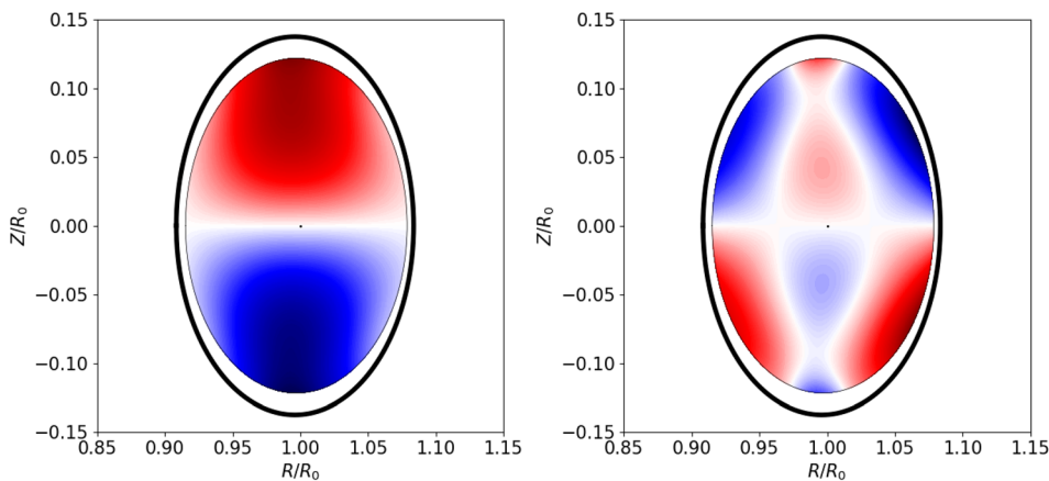
FIG. 2. The radial plasma displacement function, y(r, \theta) = f \xi^r (left panel), and the perturbed poloidal magnetic field function, Z(r, \theta) = -b_\theta (right panel), of the vertical mode for the case H_2(a) = 2 that features in Fig. 1. Here, red is positive and blue is negative. The thick black line indicates the wall.
