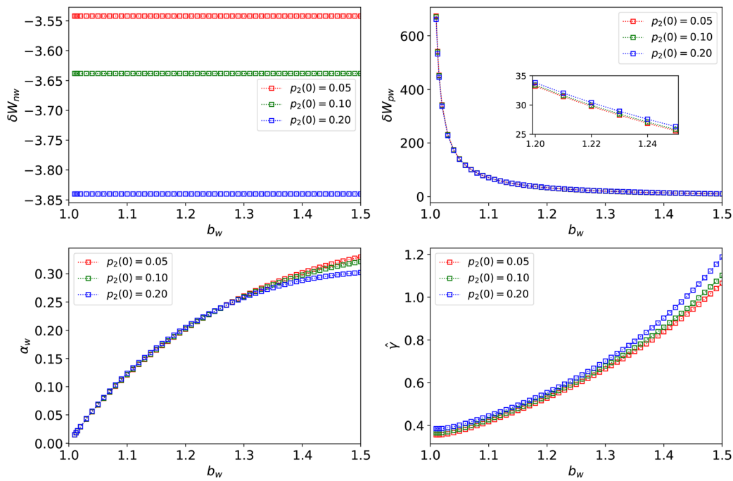
FIG. 6. The no-wall perturbed potential energy, \delta W_{nw} , the perfect-wall perturbed potential energy, \delta W_{pw} , the wall parameter, \alpha_w , and the normalized thin-wall growth-rate, \hat{\gamma} , of the vertical mode, plotted as functions of the relative wall radius, b_w , for plasma equilibria characterized by \epsilon = 0.1 , H_2(a) = 1 , H_3(a) = 0 , q(0) = 1.01 , q(a) = 3.6 , \nu_p = 2.5 , and various different values of p_2(0) .
