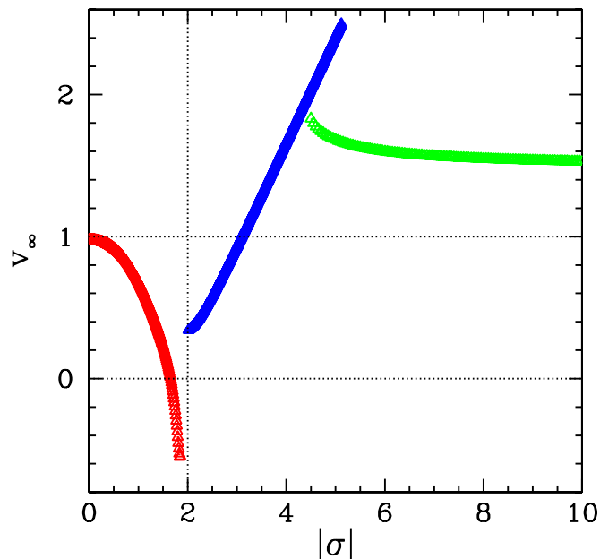
FIG. 7. (Color online) The island phase velocity parameter, v_\infty , calculated as a function of the local \mathbf{E} \times \mathbf{B} flow shear parameter, \sigma , for \alpha=2.0 , \tau=1.0 , \zeta=1.0 , and \epsilon=10^{-2} . The red (left), blue (middle), and green (right) curves correspond to the weak, intermediate, and strong flow shear regimes, respectively.
