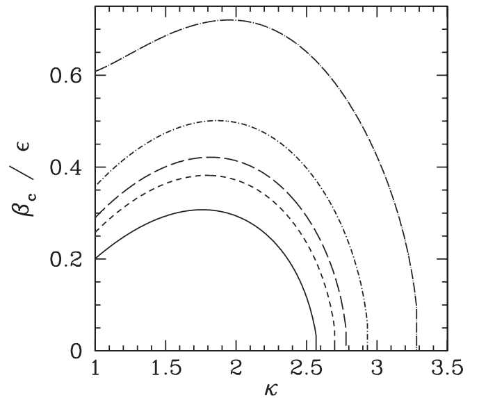
FIG. 2. \beta -limit for ideal n=1 stability vs \kappa for plasma equilibria with q_a = 2.0 . The solid, short-dashed, long-dashed, and dot-short-dashed, and dot-long-dashed curves correspond to r_w = 10.0, 1.6, 1.5, 1.4, and 1.3 , respectively. The stable region lies below the curves.
