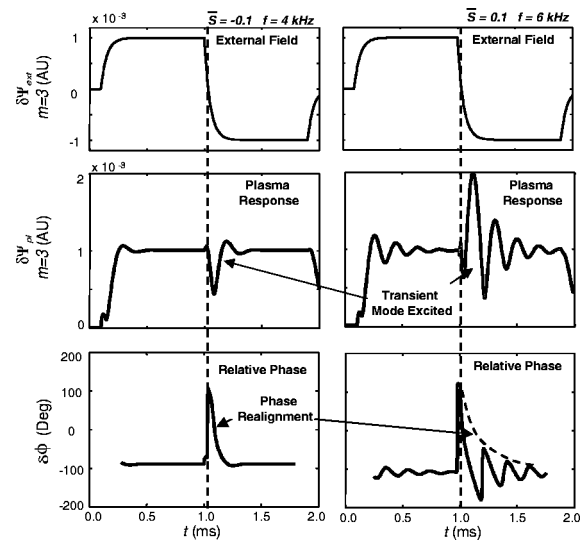
FIG. 7. Results of numerical simulations of the phase-flip experiments with Fitzpatrick–Aydemir equations for \nu_d \tau_w^* \approx 90 and for two values of stability parameter ( \bar{S} = -0.1, 0.1 ) and plasma rotation ( \Omega_0 = 4 kHz, 6 kHz).
