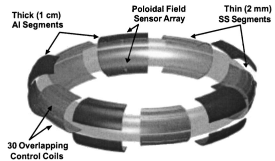
FIG. 1. Illustration of the HBT-EP experiment showing the arrangement of 20 adjustable wall segments, half of which are made of thick aluminum and half from relatively thin stainless steel. Thirty overlapping control coils are mounted on the stainless steel segments on the side not facing the plasma. A poloidal array of Mirnov sensors is decoupled from the fields of the control coils.
