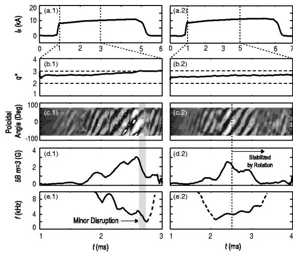
FIG. 2. Two examples of the natural growth of the RWM instability in HBT-EP. Shown parameters are: (a) total toroidal plasma current, (b) edge safety factor, (c) image of the poloidal magnetic field fluctuations at the wall measured with the poloidal Mirnov array, (d) amplitude of m=3 component of the poloidal magnetic field fluctuation at the wall, and (e) toroidal rotation rate of the magnetic field fluctuations. The discharge shown on the left shows the RWM as the q^* approaches 3. In this case, the electromagnetic torque applied to the plasma from eddy-currents in the wall reduced the mode rotation rate and a large-amplitude RWM causes a minor disruption. The discharge on the right shows a discharge where the RWM remained near marginal stability. In this case, the mode rotation increases and stabilizes the RWM.
