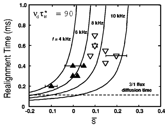
FIG. 8. Measurement of the phase realignment times in phase-flip experiments plotted versus the stability parameter, \bar{S} , early in the discharges (solid triangles) and later (open triangles). And inverse RWM damping rate predicted by Fitzpatrick–Aydemir equations (solid lines) for four different plasma rotation rates.
