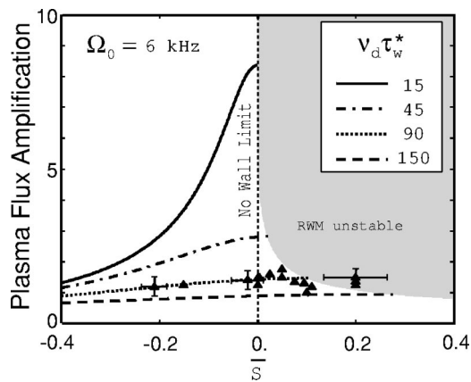
FIG. 4. The amplitude of the plasma response to a static external perturbation predicted for HBT-EP using Ref. 16 for a range of dissipation parameters and experimental measurements plotted as a function of the estimated stability parameter, \bar{S} .
