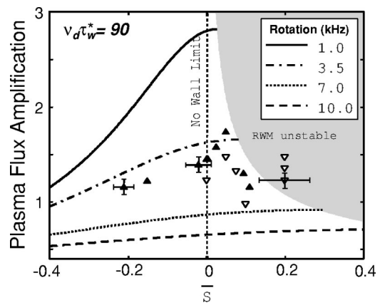
FIG. 5. The amplitude of the plasma response to a static perturbation for fixed dissipation parameter as a function of \bar{S} for a typical range of natural mode rotation rates (solid and dashed lines). Measurements of the amplitude of the plasma response taken early (solid triangles) and later (open triangles) in the discharges.
