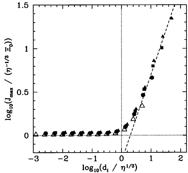
FIG. 7. Scaling of the normalized peak magnetic reconnection rate, J_{\max}/\eta^{-1/3} , with the normalized collisionless ion skin depth, d_i/\eta^{1/3} , in the linear regime. Calculations performed with L=8.0 , \tau=1.0 , \mu_i=0.0 , \nu=0.0 , and \Xi_0=10^{-4} . The solid triangular data points correspond to \eta=10^{-6} . The solid square data points correspond to \eta=10^{-5} . The solid circular data points correspond to \eta=10^{-4} . The open triangular data points correspond to \eta=10^{-3} . The dashed line is a fit to J_{\max}/\eta^{-1/3} \propto d_i/\eta^{1/3} .
