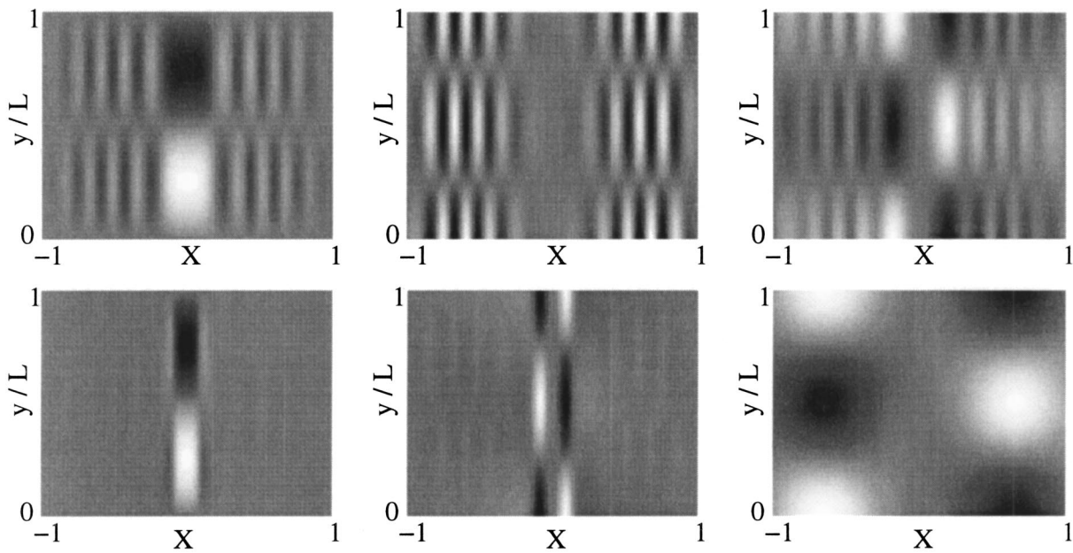
FIG. 2. Typical current density, etc., patterns associated with forced reconnection in the linear MHD and linear Hall-MHD regimes. Calculations performed with L=8.0 , \tau=1.0 , \eta=10^{-4} , \mu_i=10^{-8} , \nu=0.0 , and \Xi_0=10^{-4} . All panels show data taken at the peak reconnection rate. The left panels show density plots of the current density, j_z . The middle panels show density plots of the out-of-plane magnetic field-strength, B_z . The right panels show density plots of the ion streamfunction, \phi . The upper panels show calculations made using d_i=10^{-3} , corresponding to the linear MHD regime. The lower panels show calculations made using d_i=1.0 , corresponding to the linear Hall-MHD regime. Note that X=\text{sgn}(x)\sqrt{|x|/(2-|x|)} is a stretched coordinate.
