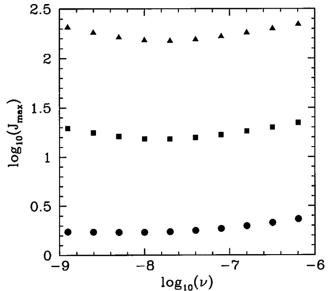
FIG. 11. Scaling of the peak magnetic reconnection rate, J_{\max} , with hyper-resistivity, \nu , in the nonlinear Hall-MHD regime. Calculations performed with L=8.0 , \tau=1.0 , \mu_i=\eta/10 , d_i=1.0 , and \Xi_0=10^{-2} . The triangular data points show \eta=10^{-6} . The square data points show \eta=10^{-5} . The circular data points show \eta=10^{-4} .
