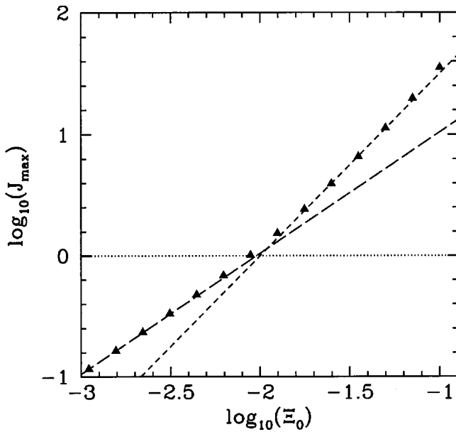
FIG. 9. Scaling of the peak magnetic reconnection rate, J_{\max} , with the perturbation amplitude, \Xi_0 , in the linear/nonlinear MHD regime. Calculations performed with L=8.0 , \tau=1.0 , \eta=10^{-6} , \mu_i=10^{-7} , \nu=0.0 , and d_i=0.0 . The long-dashed line is a fit to J_{\max} \propto \Xi_0^1 . The short-dashed line is a fit to J_{\max} \propto \Xi_0^{3/2} .
