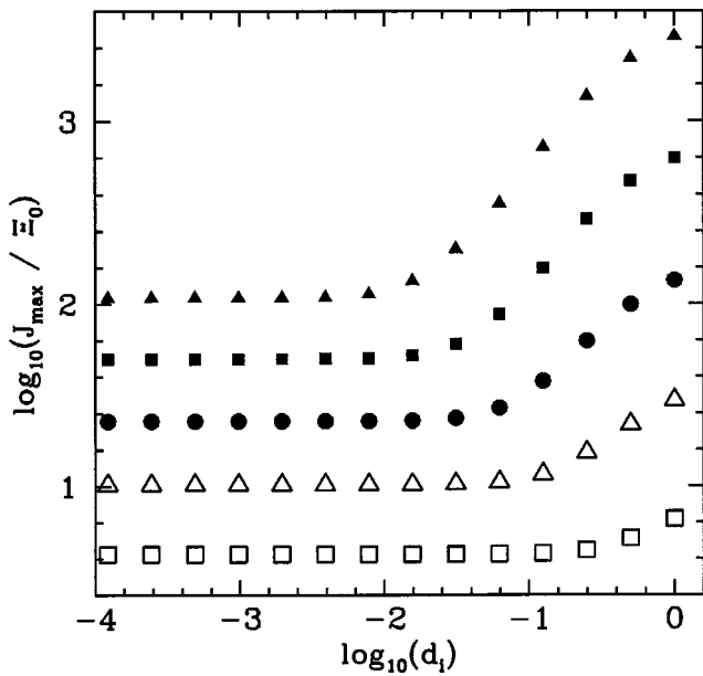
FIG. 6. Scaling of the peak magnetic reconnection rate, J_{\max} , with the collisionless ion skin depth, d_i , in the linear regime. Calculations performed with L=8.0 , \tau=1.0 , \mu_i=0.0 , \nu=0.0 , and \Xi_0=10^{-4} . The solid triangular data points correspond to \eta=10^{-6} . The solid square data points correspond to \eta=10^{-5} . The solid circular data points correspond to \eta=10^{-4} . The open triangular data points correspond to \eta=10^{-3} . The open square data points correspond to \eta=10^{-2} .
