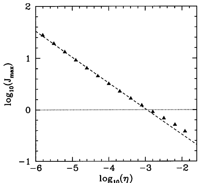
FIG. 8. Scaling of the peak magnetic reconnection rate, J_{\max} , with resistivity, \eta , in the linear/nonlinear MHD regime. Calculations performed with L=8.0 , \tau=1.0 , \mu_i=\eta/10 , \nu=0.0 , d_i=0.0 , and \Xi_0=0.1 . The dashed line is a fit to J_{\max} \propto \eta^{-1/2} .
