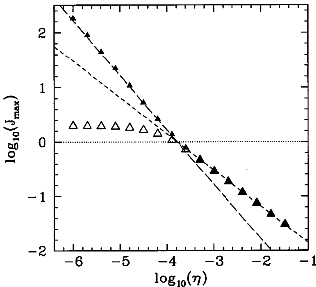
FIG. 10. Scaling of the peak magnetic reconnection rate, J_{\max} , with resistivity, \eta , in the linear/nonlinear Hall-MHD regime. Calculations performed with L=8.0 , \tau=1.0 , \mu_i=\eta/10 , \nu=2.5 \times 10^{-9} , d_i=1.0 , and \Xi_0=10^{-2} . The solid data points show the total reconnection rate. The open data points show the resistive contribution to the reconnection rate. The short-dashed line is a fit to J_{\max} \propto \eta^{-2/3} . The long-dashed line is a fit to J_{\max} \propto \eta^{-1} .
