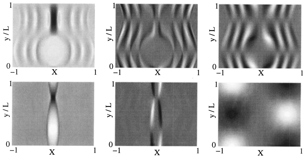
FIG. 3. Typical current density, etc., patterns associated with forced reconnection in the nonlinear MHD and nonlinear Hall-MHD regimes. Calculations performed with L=8.0 , \tau=1.0 , \eta=10^{-5} , and \mu_i=10^{-6} . All panels show data taken at the peak reconnection rate. The left panels show density plots of the current density, j_z . The middle panels show density plots of the out-of-plane magnetic field-strength, B_z . The right panels show density plots of the ion streamfunction, \phi . The upper panels show calculations made using d_i=10^{-3} , \nu=0.0 , and \Xi_0=0.1 , corresponding to the nonlinear MHD regime. The lower panels show calculations made using d_i=1.0 , \nu=2.5 \times 10^{-9} , and \Xi_0=10^{-2} , corresponding to the nonlinear Hall-MHD regime. Note that X=\text{sgn}(x)\sqrt{|x|/(2-|x|)} is a stretched coordinate.
