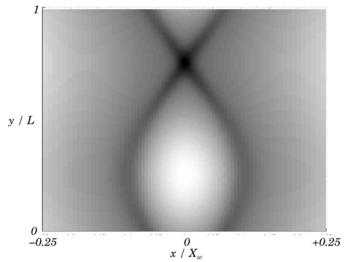
FIG. 7. A plot of the current density, j(x,y) , at t=1000 for the simulation shown in Figs. 5 and 6. Dark areas correspond to more positive j values and vice versa. The magnetic O-point is located at (0, 0.25 L) , whereas the X-point is located at (0, 0.75 L) .
