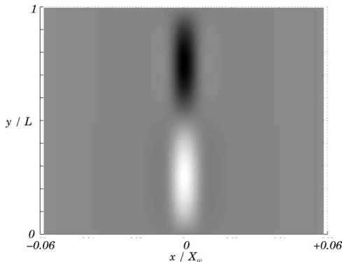
FIG. 10. A plot of the current density, j(x,y) , at t = 300 for a simulation with \eta = 1 \times 10^{-7} , \mu = 1 \times 10^{-6} , \Xi_0 = 4 \times 10^{-3} , and \tau_{\text{on}} = 10 . Dark areas correspond to more positive j values and vice versa . The magnetic O-point is located at (0, 0.25 L) , whereas the X-point is located at (0, 0.75 L) .
