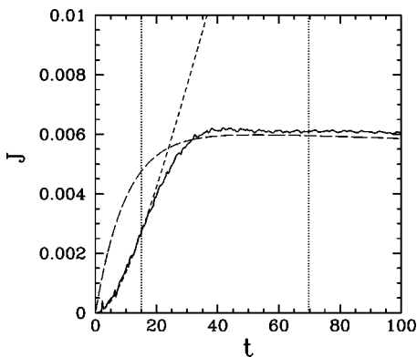
FIG. 2. The reconnection rate, J(t) (solid curve) versus time for a simulation with X_w = 1.5 , L = 3.0 , \eta = 1 \times 10^{-5} , \mu = 1 \times 10^{-4} , \Xi_0 = 1 \times 10^{-3} , and \tau_{on} = 10 . The leftmost vertical dotted line indicates when t = \tau_1 , whereas the rightmost line shows when t = \tau_2 . The short-dashed curve shows the theoretical reconnection rate in the inertial regime, J_I(t) . The long-dashed curve shows the theoretical reconnection rate in the visco-resistive regime, J_{VR}(t) .
