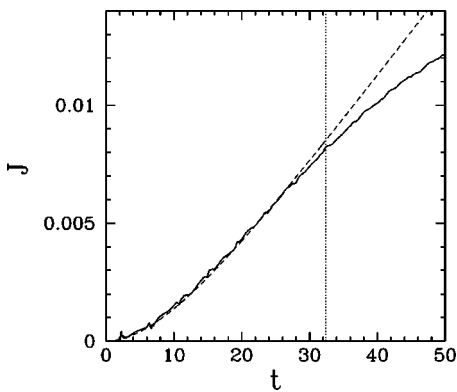
FIG. 1. The reconnection rate, J(t) (solid curve) versus time for a simulation with X_w = 1.5 , L = 3.0 , \eta = 1 \times 10^{-6} , \mu = 1 \times 10^{-5} , \Xi_0 = 1 \times 10^{-3} , and \tau_{on} = 10 . The vertical dotted line indicates when t = \tau_1 . The dashed curve shows the theoretical reconnection rate in the inertial regime, J_I(t) .
