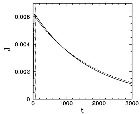
FIG. 3. The reconnection rate, J(t) (solid curve) versus time for a simulation with X_w = 1.5 , L = 3.0 , \eta = 1 \times 10^{-5} , \mu = 1 \times 10^{-4} , \Xi_0 = 1 \times 10^{-3} , and \tau_{on} = 10 . The vertical dotted vertical line indicates when t = \tau_2 . The dashed curve shows the theoretical reconnection rate in the visco-resistive regime, J_{VR}(t) .
