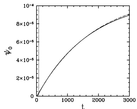
FIG. 4. The reconnected flux, \psi_0(t) (solid curve) versus time for a simulation with X_w = 1.5 , L = 3.0 , \eta = 1 \times 10^{-5} , \mu = 1 \times 10^{-4} , \Xi_0 = 1 \times 10^{-3} , and \tau_{on} = 10 . The vertical dotted vertical line indicates when t = \tau_2 . The dashed curve shows the theoretical reconnected flux in the visco-resistive regime, \psi_{VR}(t) .
