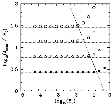
FIG. 9. The maximum reconnection rate, J_{\max} , divided by the perturbation amplitude, \Xi_0 , plotted versus the perturbation amplitude. All simulations have X_w = 1.5 , L = 3.0 , and \tau_{\text{on}} = 10 . The open circles show simulations with \eta = 1 \times 10^{-7} and \mu = 1 \times 10^{-6} . The open squares show simulations with \eta = 1 \times 10^{-6} and \mu = 1 \times 10^{-5} . The open triangles show simulations with \eta = 1 \times 10^{-5} and \mu = 1 \times 10^{-4} . The solid circles show simulations with \eta = 1 \times 10^{-4} and \mu = 1 \times 10^{-3} . The dotted horizontal lines show the corresponding theoretical J_{\max}/\Xi_0 values in the absence of a Sweet–Parker reconnection phase [see Eq. (58)]. The dashed diagonal line corresponds to J_{\max} = 0.5 .
