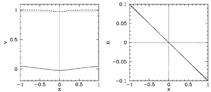
FIG. 11. Left-hand panel: The electron fluid (dashed curve) and ion fluid (solid curve) velocity profiles, v_e and v_i , through the O point, calculated for an electron branch island close to the bifurcation to the ion branch. The island-phase velocity, v , is indicated by the horizontal dotted line. The calculation parameters are \rho=1.745 \times 10^{-1} , L_s/L_n=10 , V_s=0.1 , k=1 , \Psi=10^{-2} , and \eta=D=\mu=\chi=7.071 \times 10^{-4} . Right-hand panel: The electron density profiles through the O (solid curve) and X points (dashed curve), calculated for the same island.
